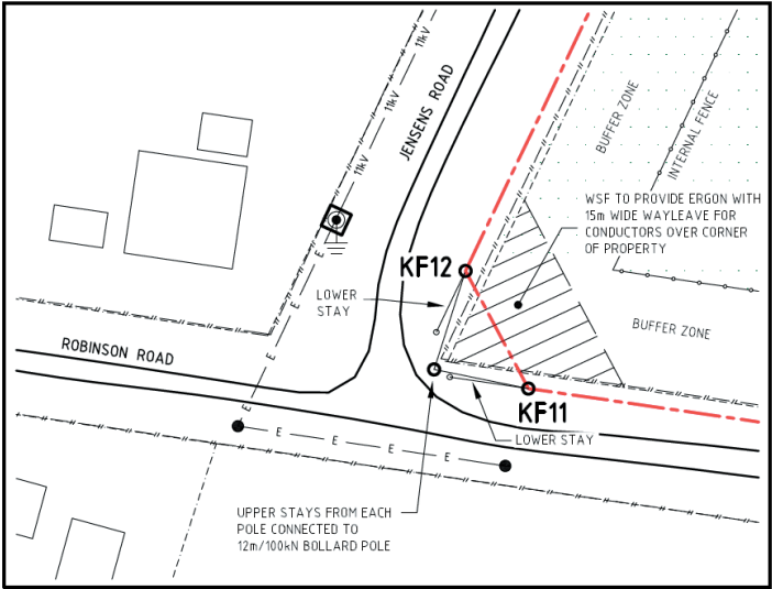
INSET DETAIL B SCALE 1: 500
